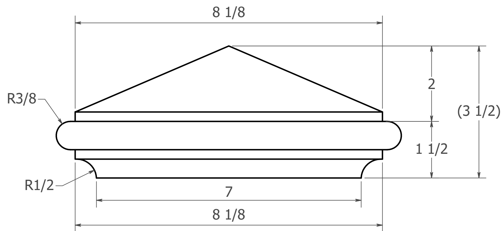
FRONT SCALE 2:3
