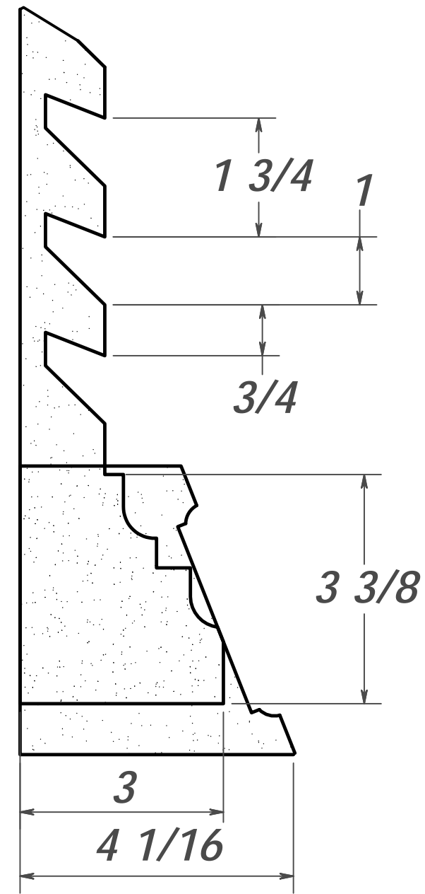
CLOSED LOUVER
