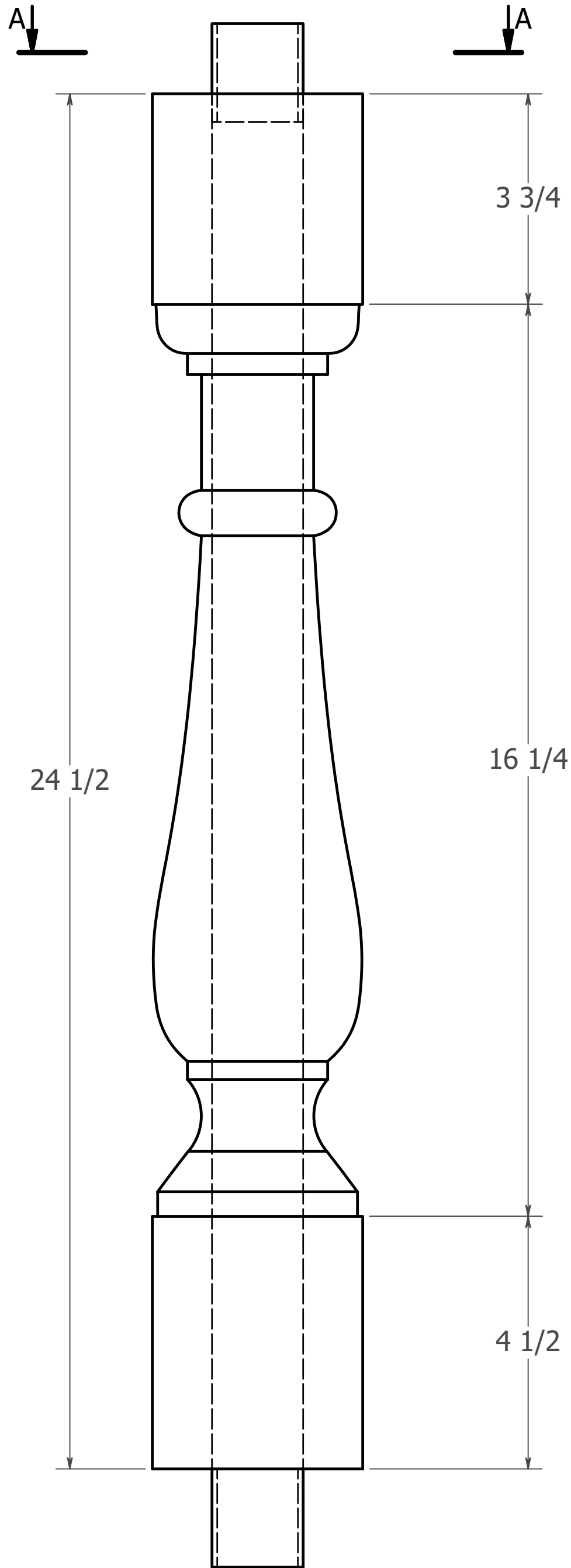
FRONT SCALE 1 / 2
