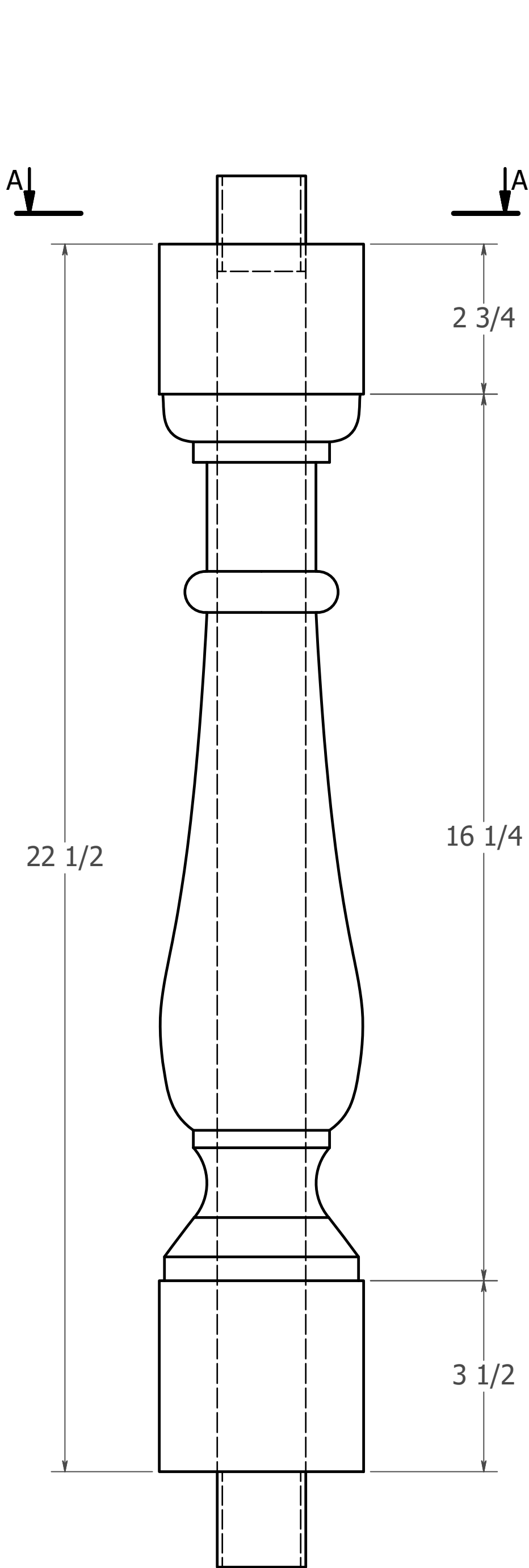
FRONT SCALE 1 / 2
