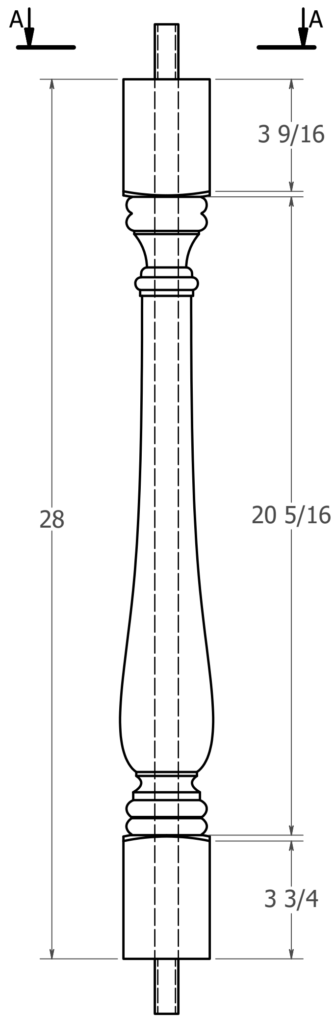
FRONT SCALE 1/3
