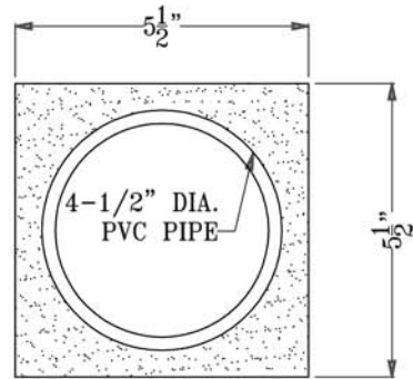
A SECTION - FLAT NEWEL POST
