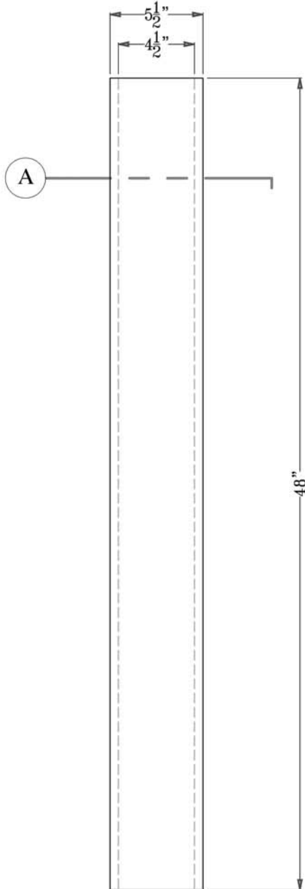
ELEVATION - FLAT NEWEL POST
